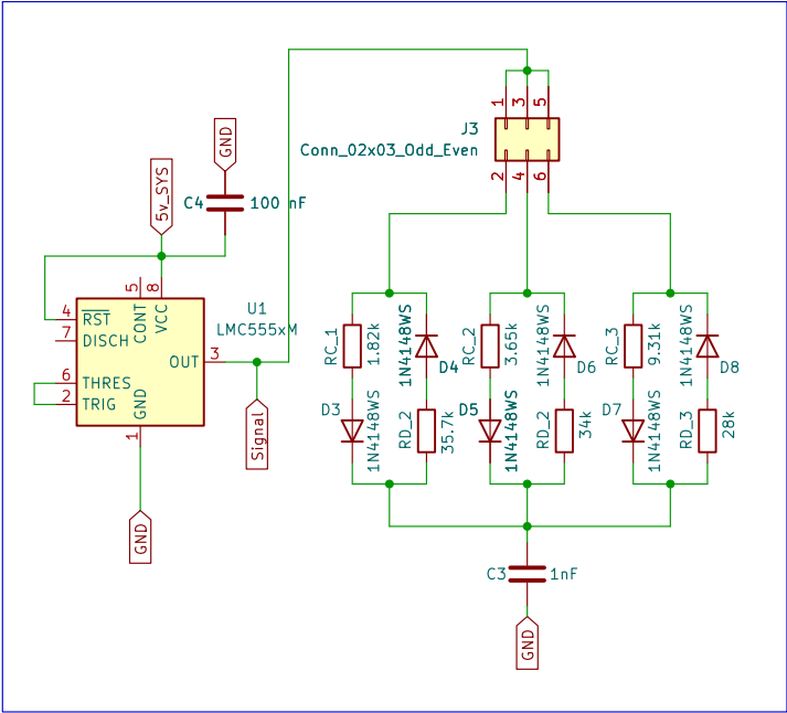
Subsystem 2 (Oscillator)
