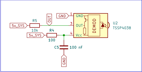
Subsystem 4 (Receiver)
