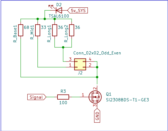
Subsystem 3 (Driver)
